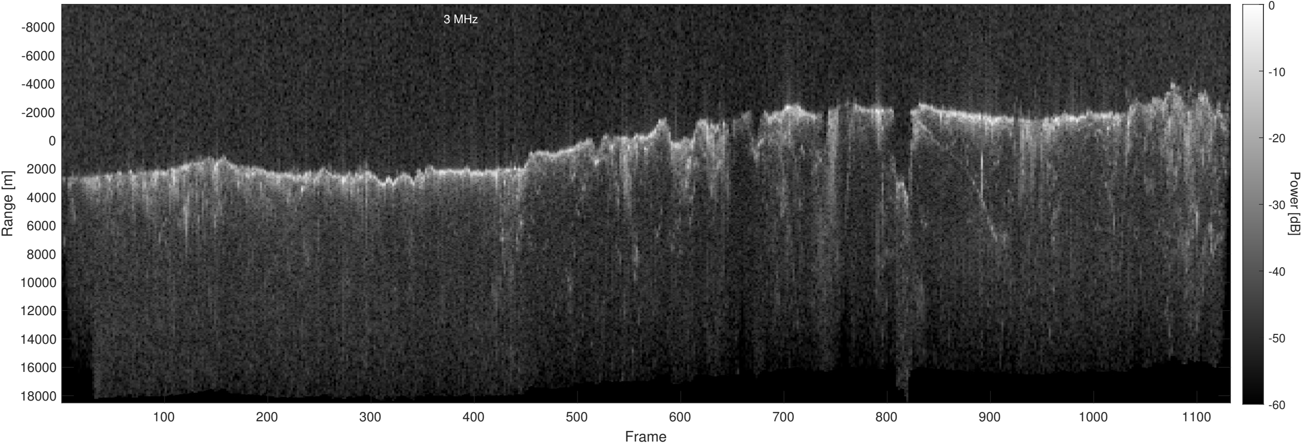
Orbit 13489, Optimized, Window, Depth-Corrected, Channel 2
