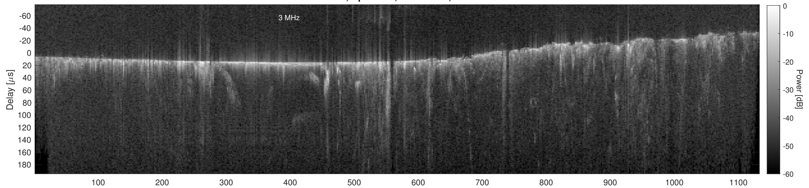
Orbit 13490, Cluttergram
