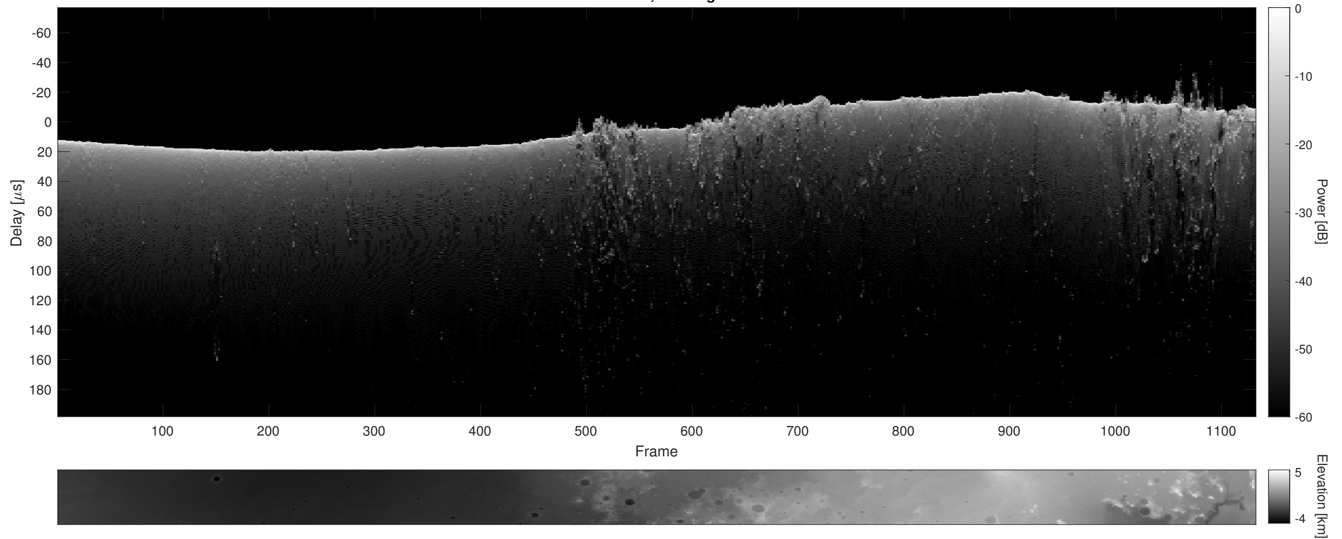
Orbit 13491, Cluttergram
