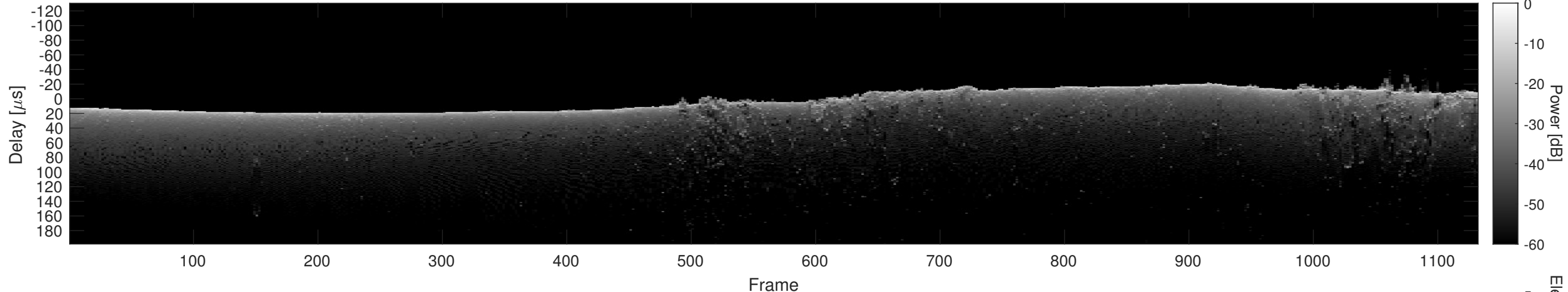
Orbit 13491, Cluttergram
