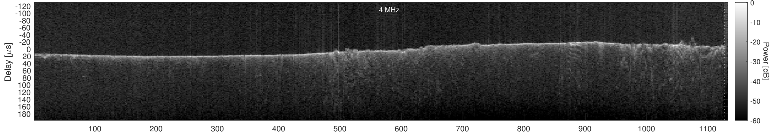
Orbit 13491, Cluttergram
