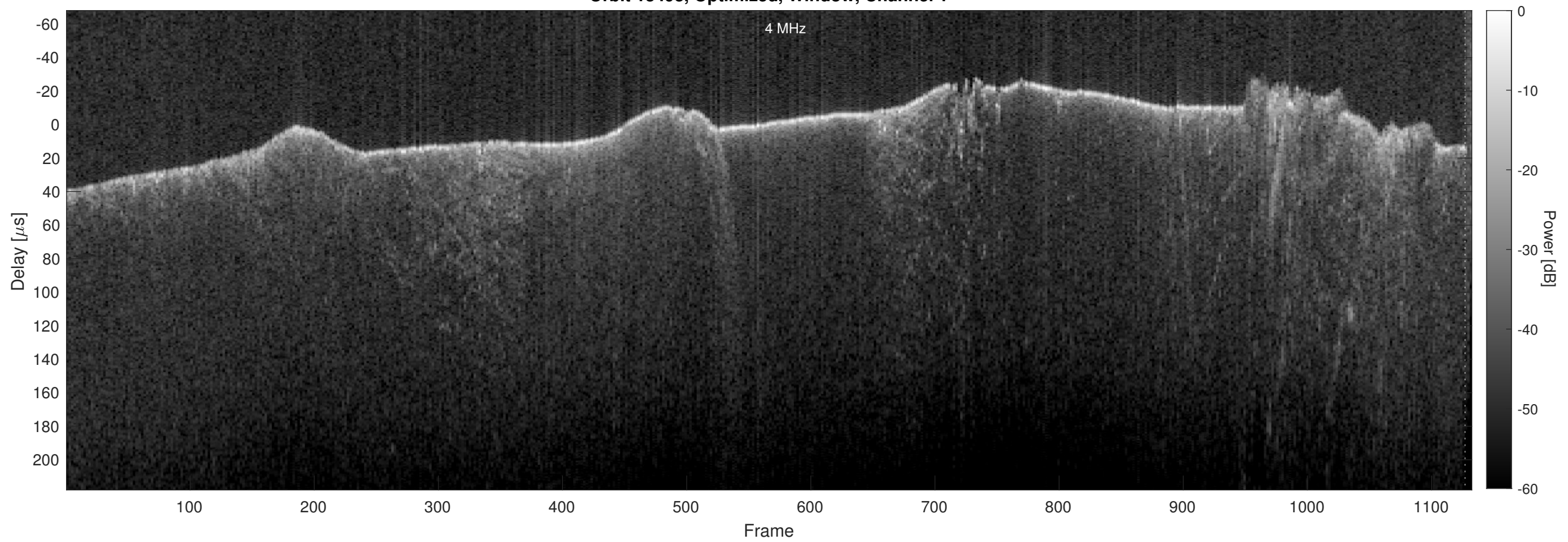
Orbit 13493, Optimized, Window, Channel 2
