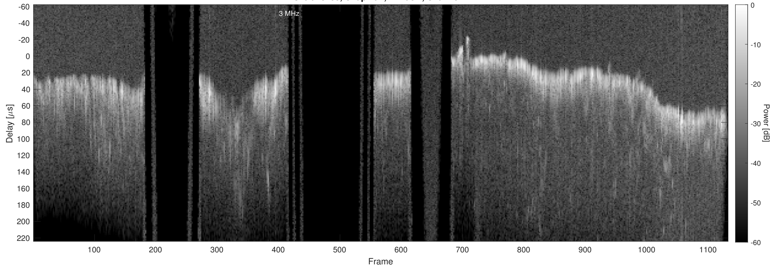
Orbit 13495, Chapman, Window, Channel 2
