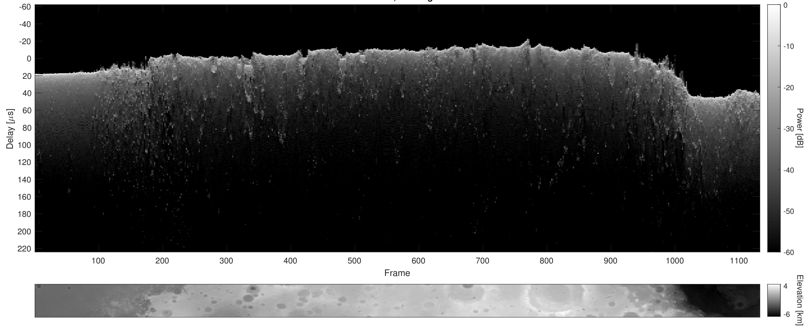
Orbit 13495, Cluttergram
