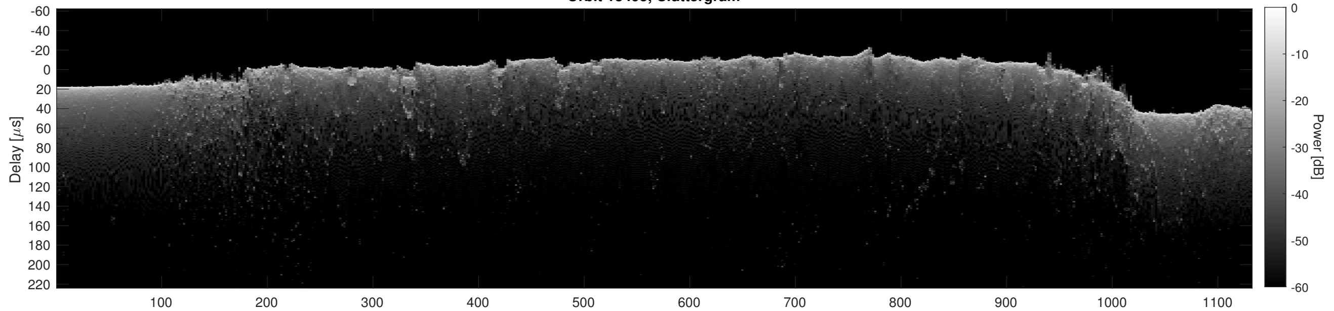
Orbit 13495, Cluttergram
