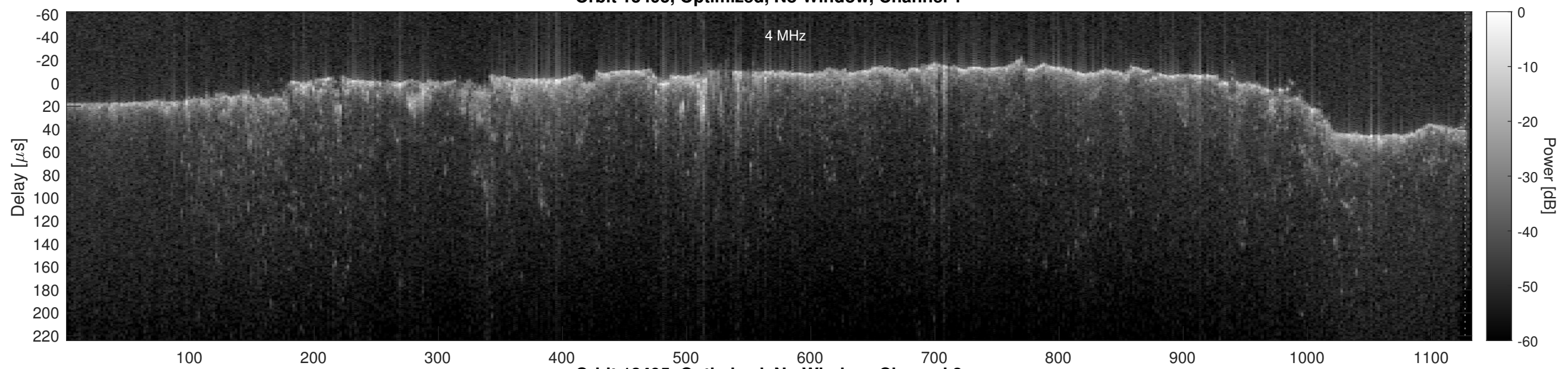
Orbit 13495, Optimized, No Window, Channel 2
