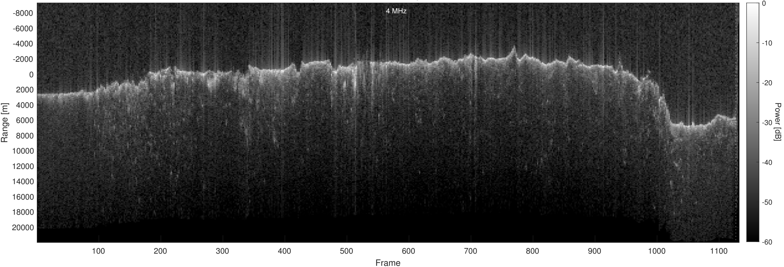
Orbit 13495, Optimized, No Window, Depth-Corrected, Channel 2
