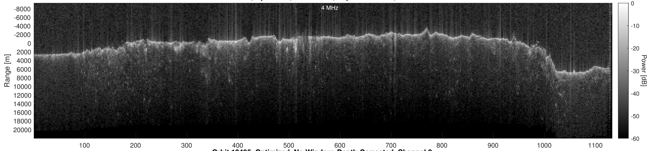
Orbit 13495, Optimized, No Window, Depth-Corrected, Channel 2
