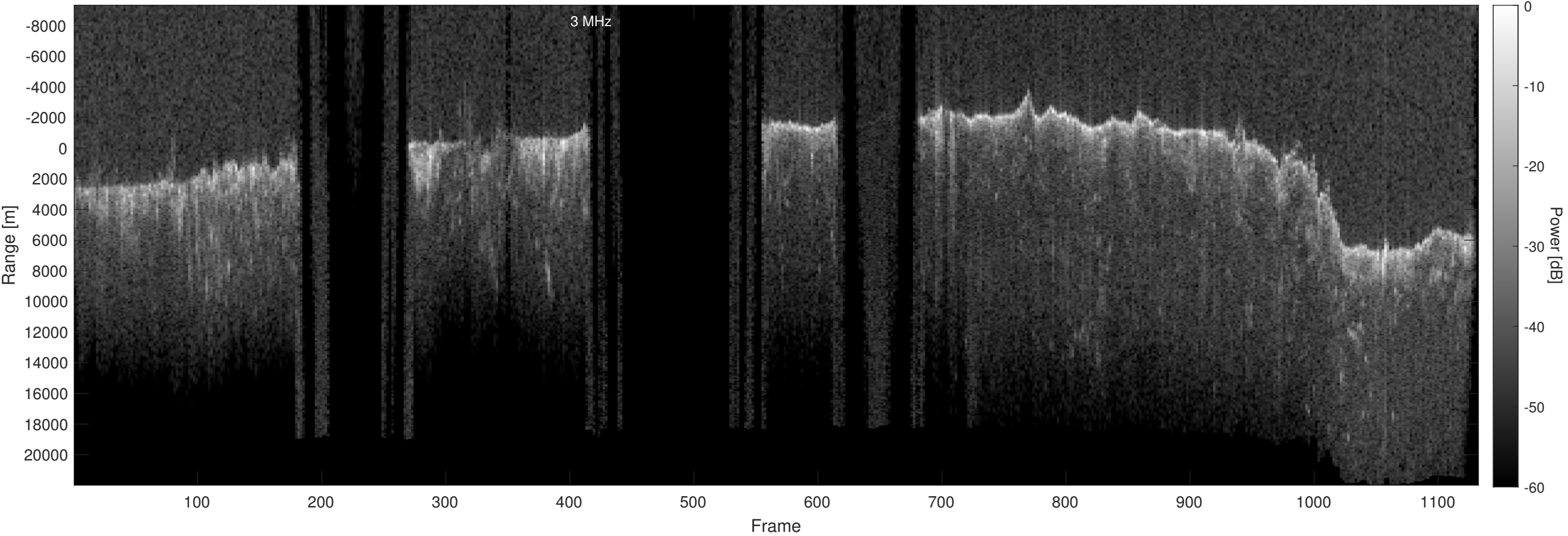
Orbit 13495, Optimized, Window, Depth-Corrected, Channel 2
