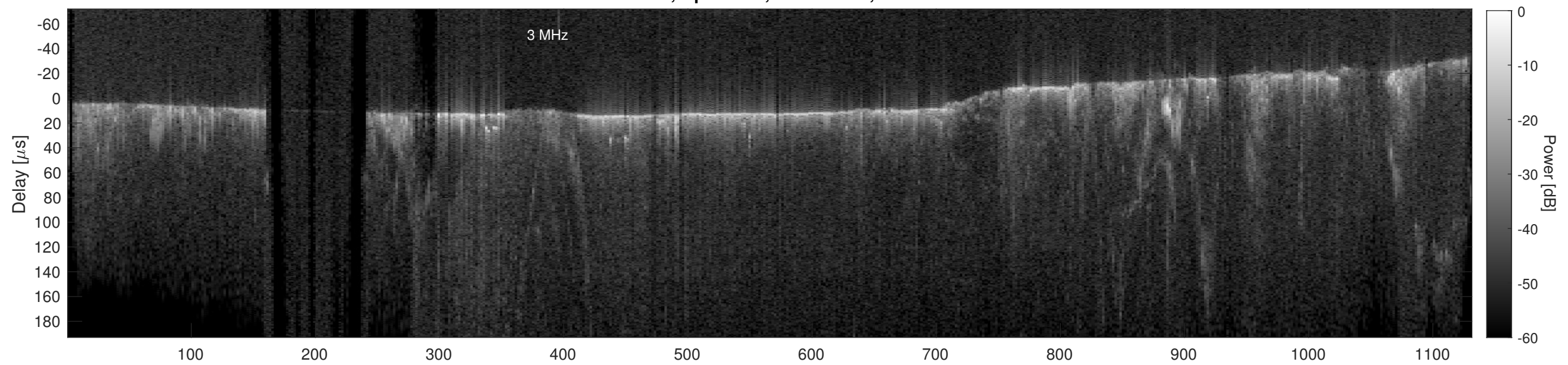
Orbit 13497, Cluttergram
