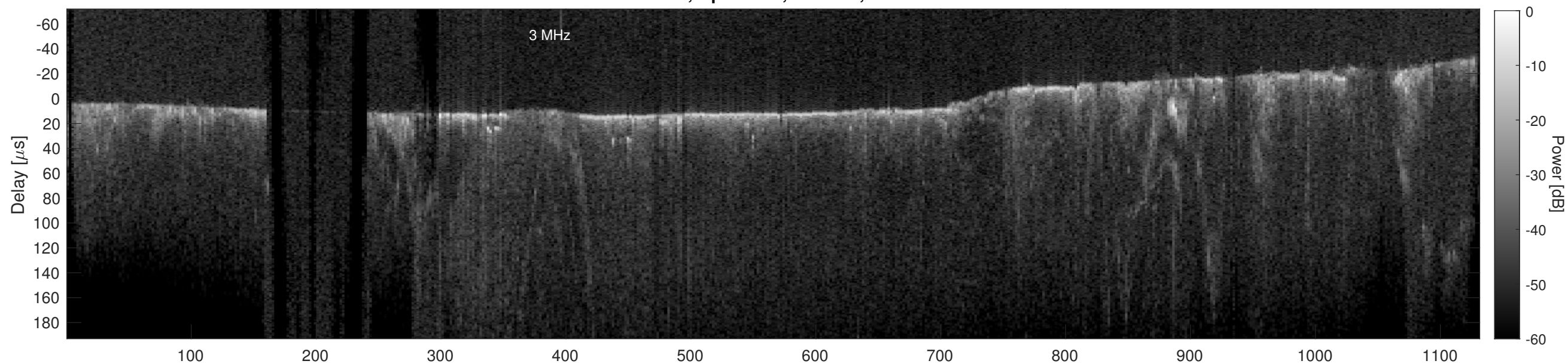
Orbit 13497, Cluttergram
