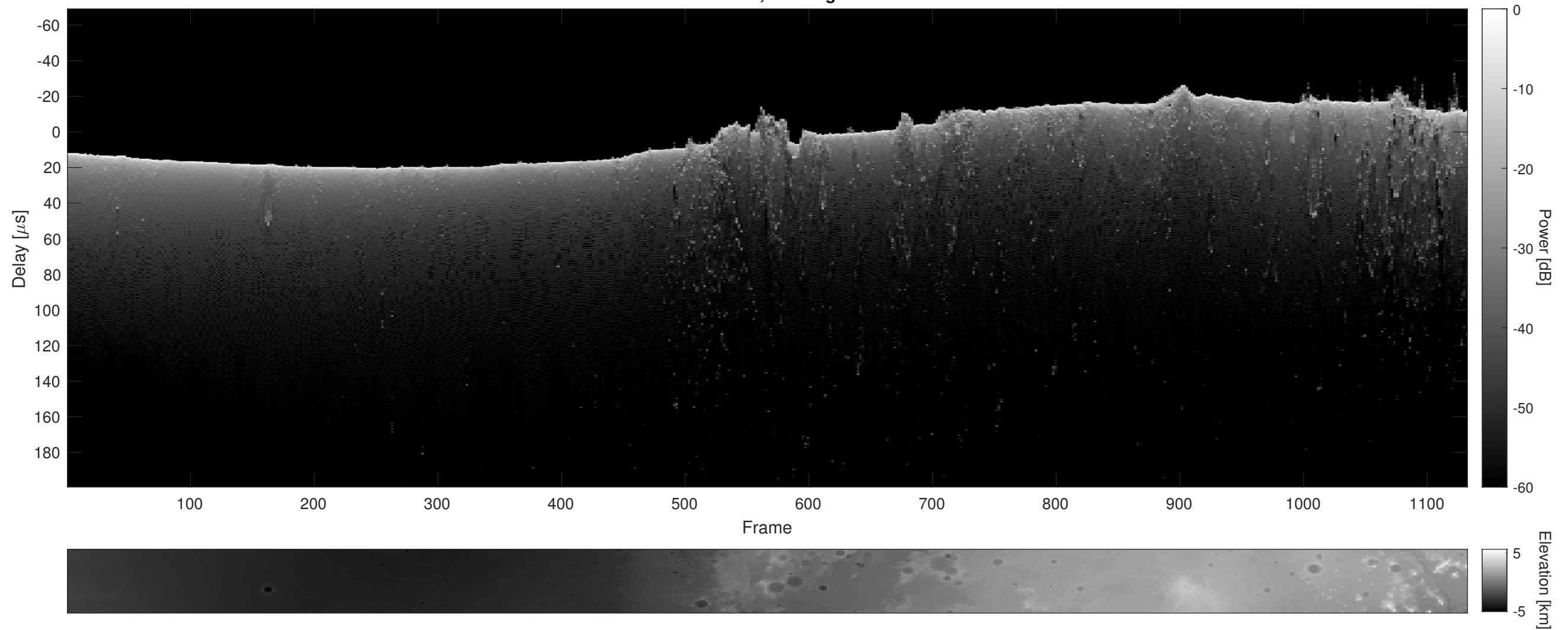
Orbit 13498, Cluttergram
