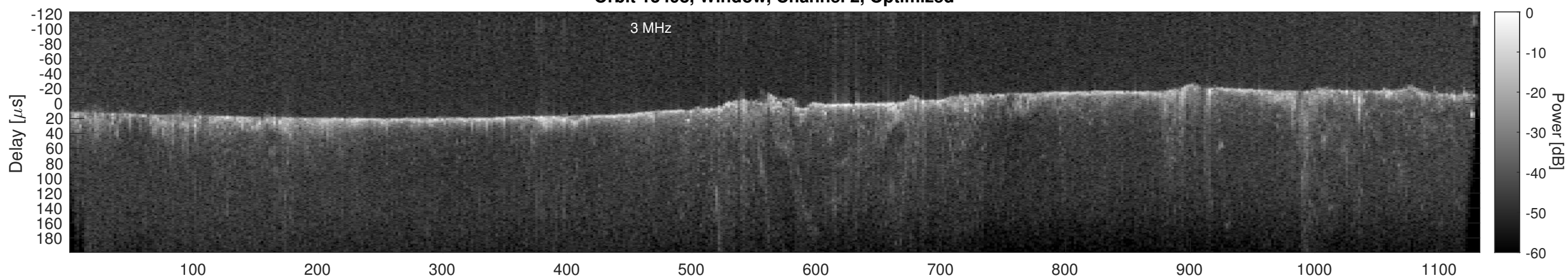
Orbit 13498, Cluttergram
