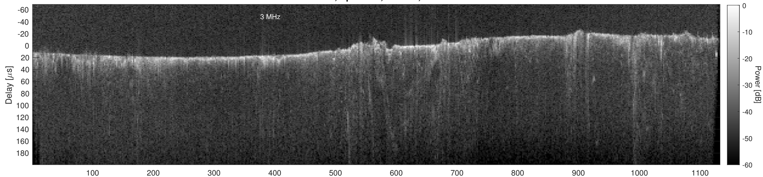
Orbit 13498, Cluttergram
