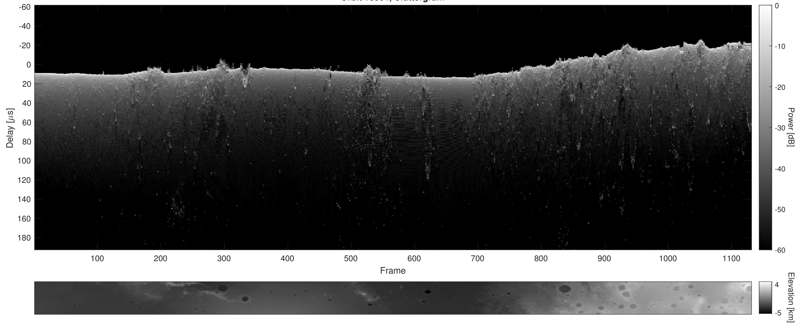
Orbit 13501, Cluttergram
