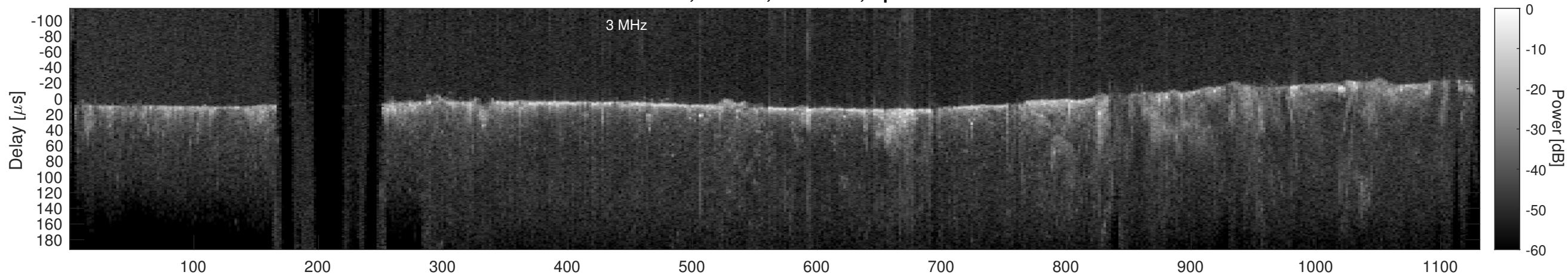
Orbit 13501, Cluttergram
