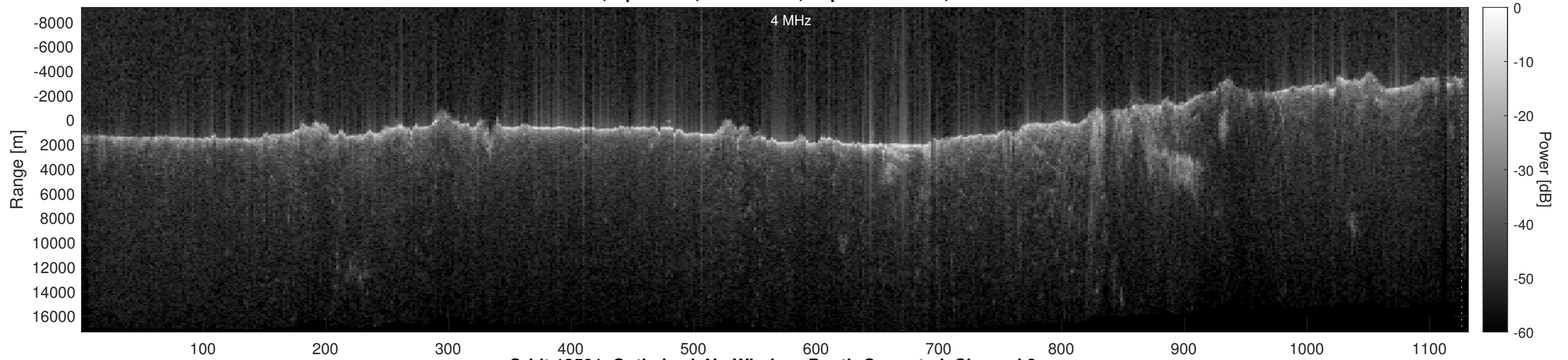
Orbit 13501, Optimized, No Window, Depth-Corrected, Channel 2
