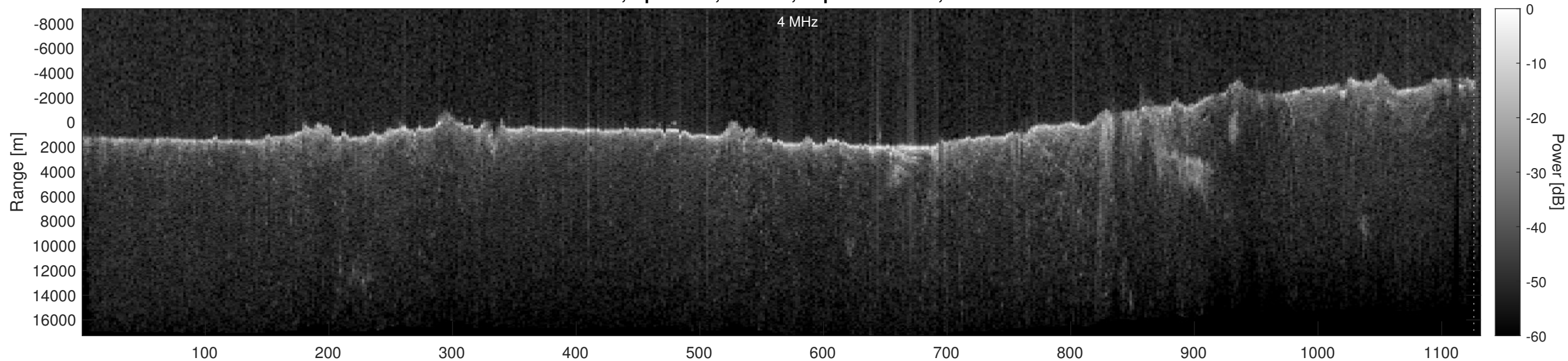
Orbit 13501, Optimized, Window, Depth-Corrected, Channel 2
