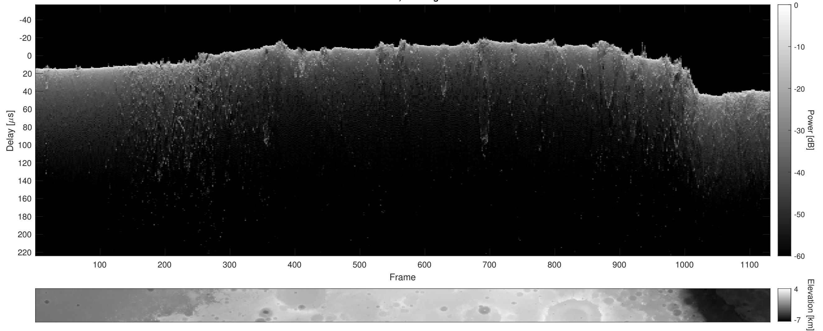
Orbit 13502, Cluttergram
