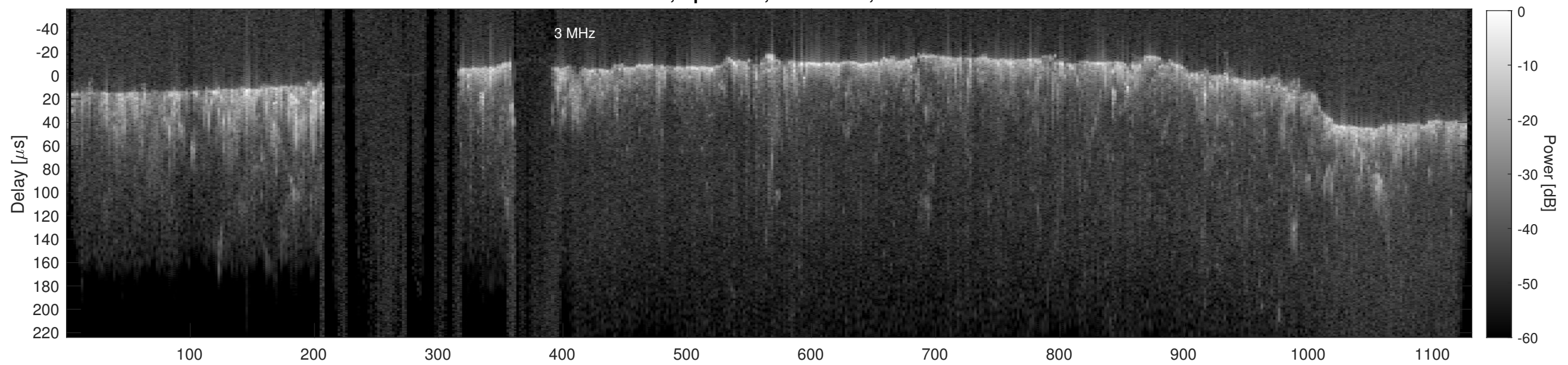
Orbit 13502, Cluttergram
