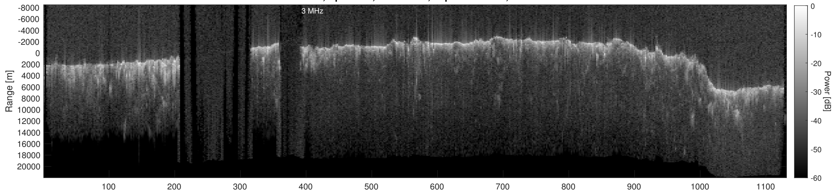
Orbit 13502, Depth-Corrected Cluttergram
