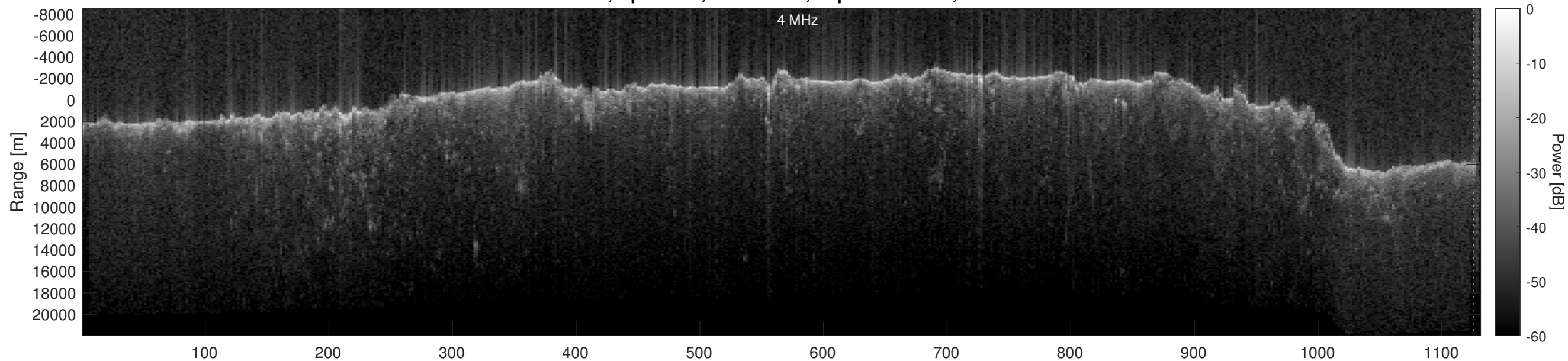
Orbit 13502, Optimized, No Window, Depth-Corrected, Channel 2
