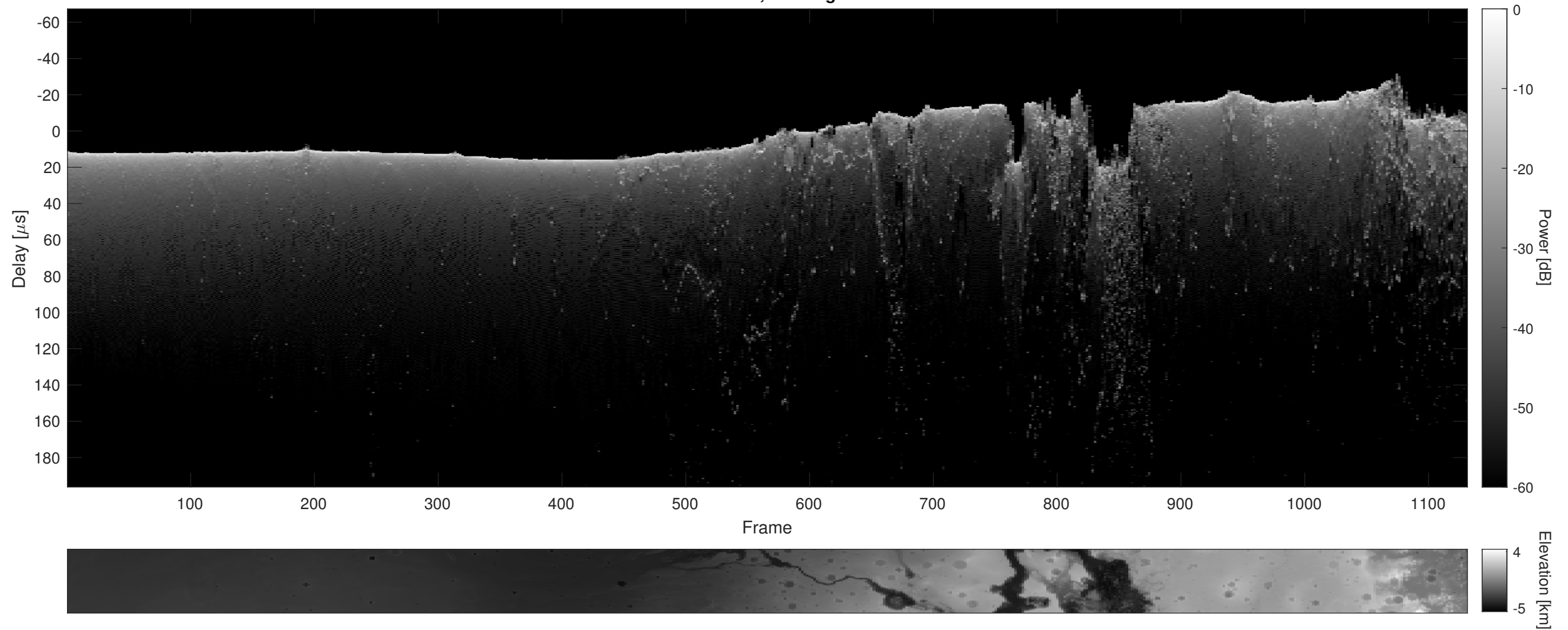
Orbit 13503, Cluttergram
