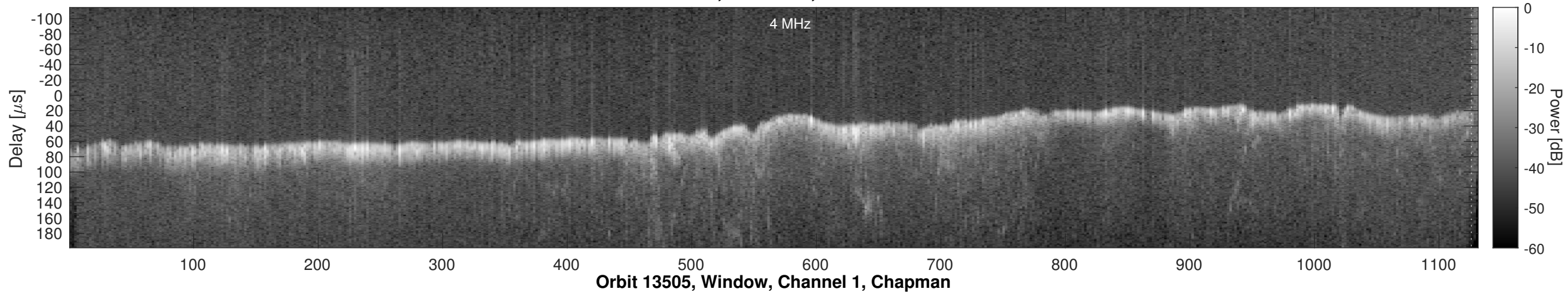
Orbit 13505, Channel 1, Uncorrected
