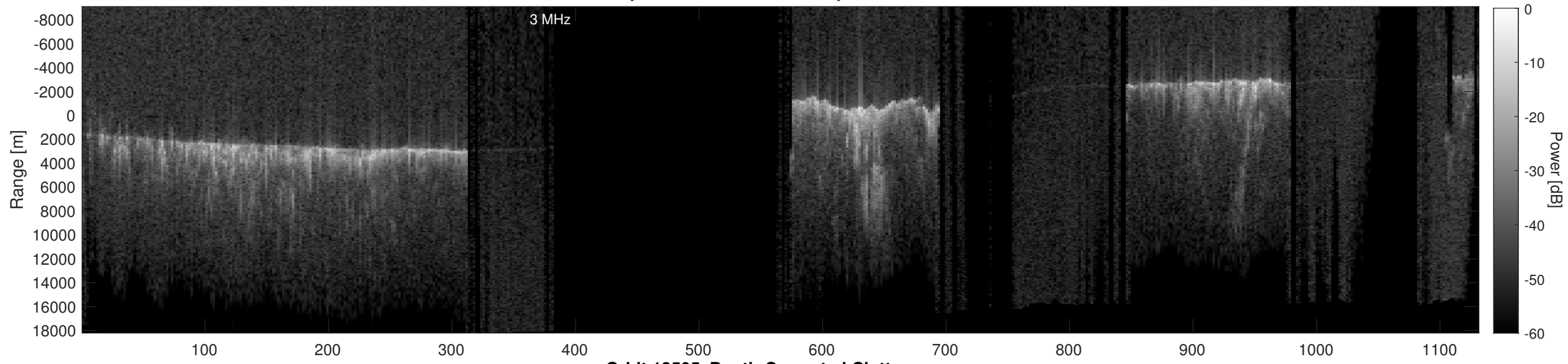
Orbit 13505, Depth-Corrected Cluttergram
