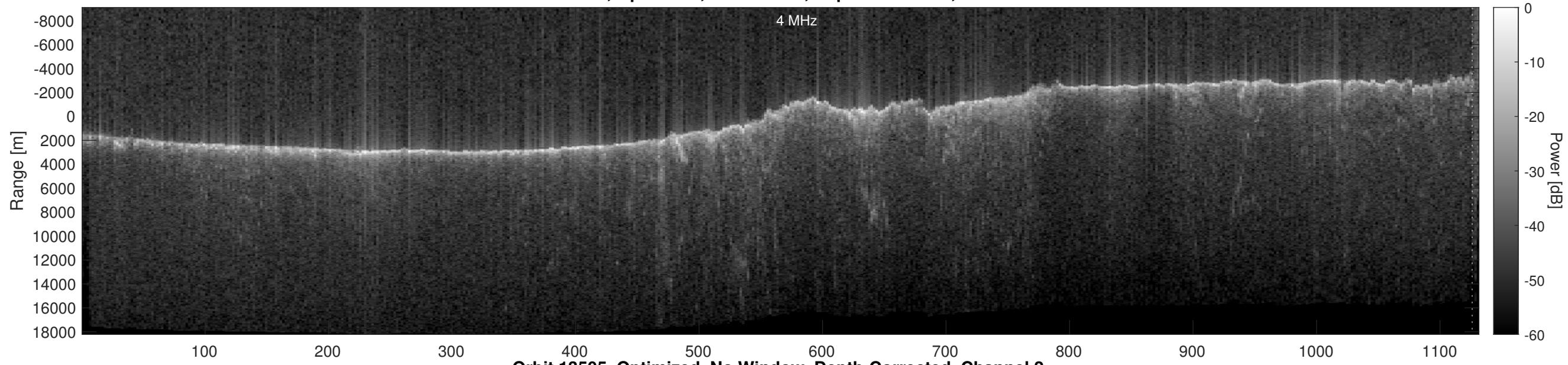
Orbit 13505, Optimized, No Window, Depth-Corrected, Channel 2
