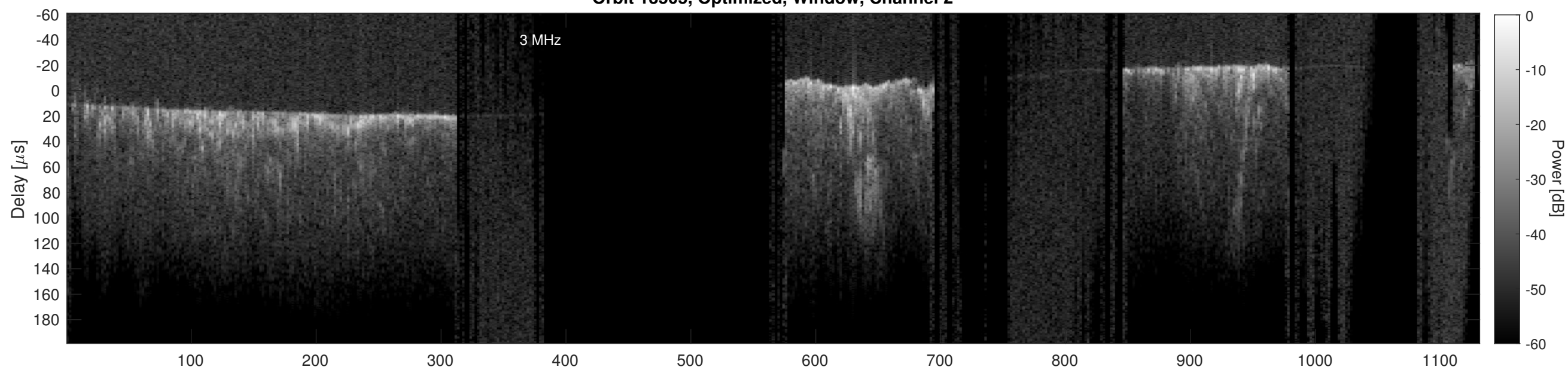
Orbit 13505, Cluttergram
