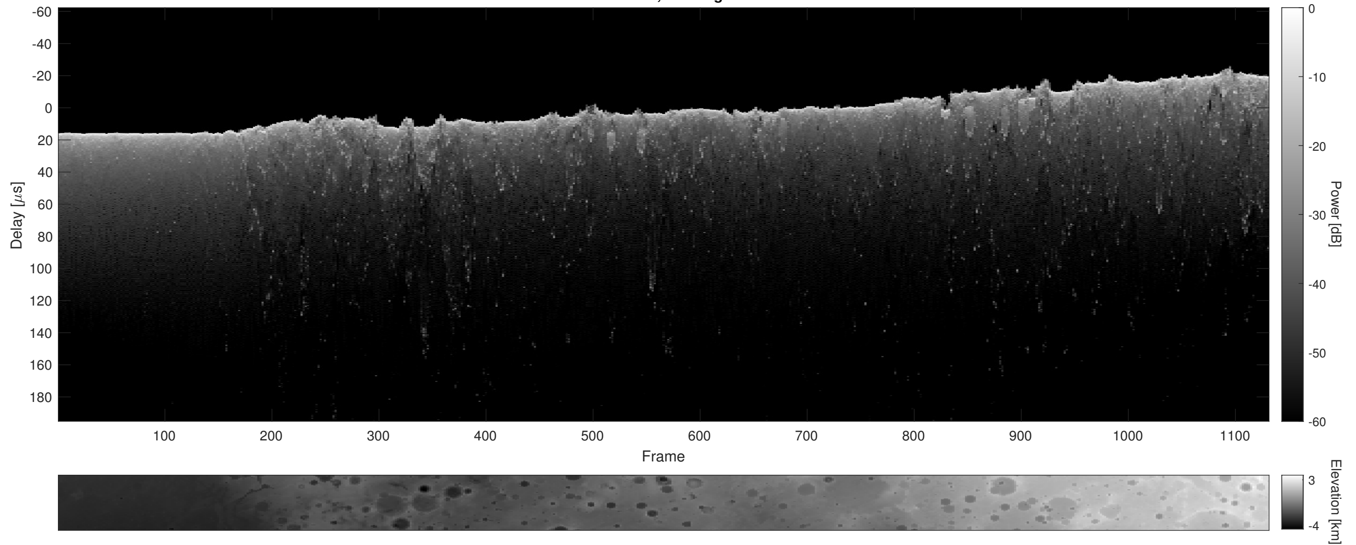
Orbit 13506, Cluttergram
