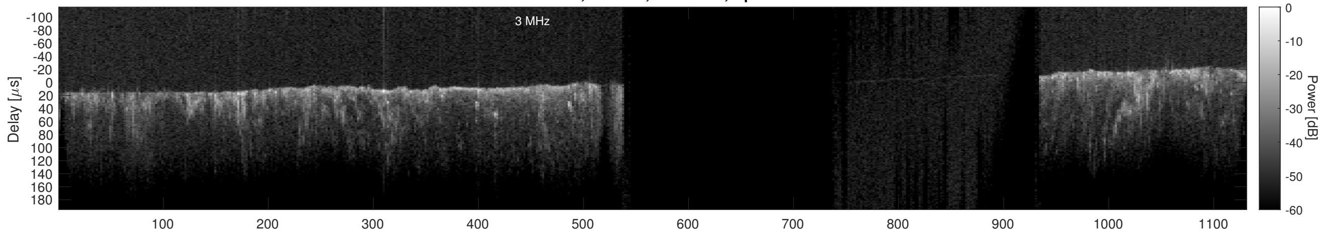
Orbit 13506, Cluttergram
