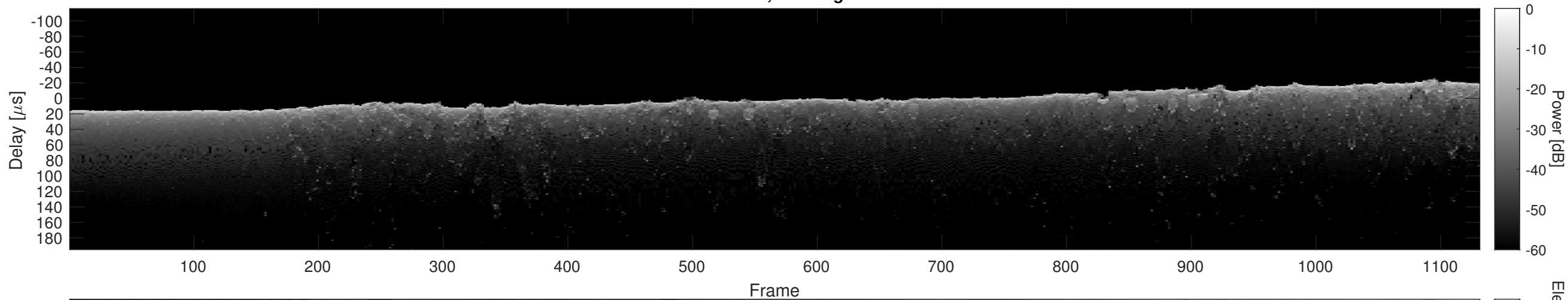
Orbit 13506, Cluttergram
