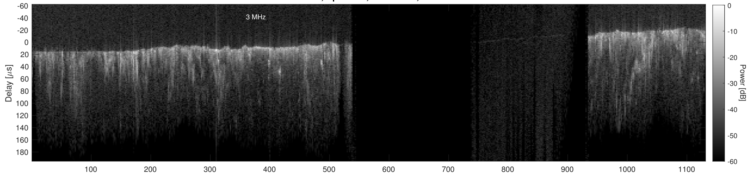
Orbit 13506, Cluttergram
