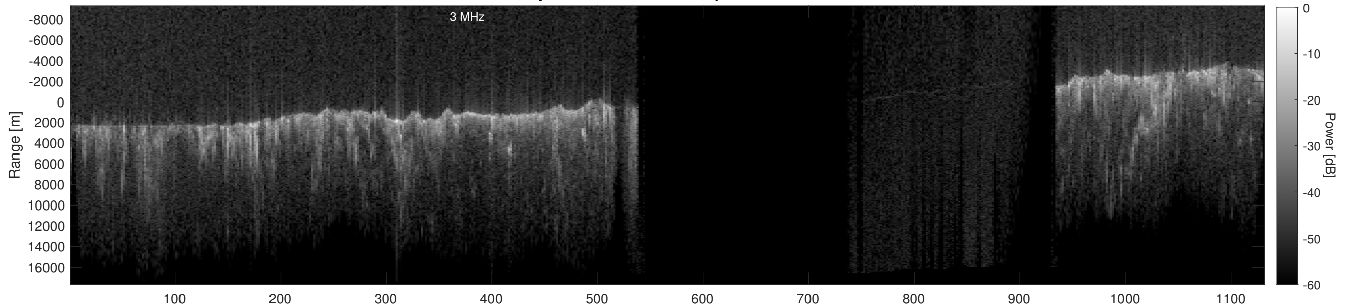
Orbit 13506, Depth-Corrected Cluttergram
