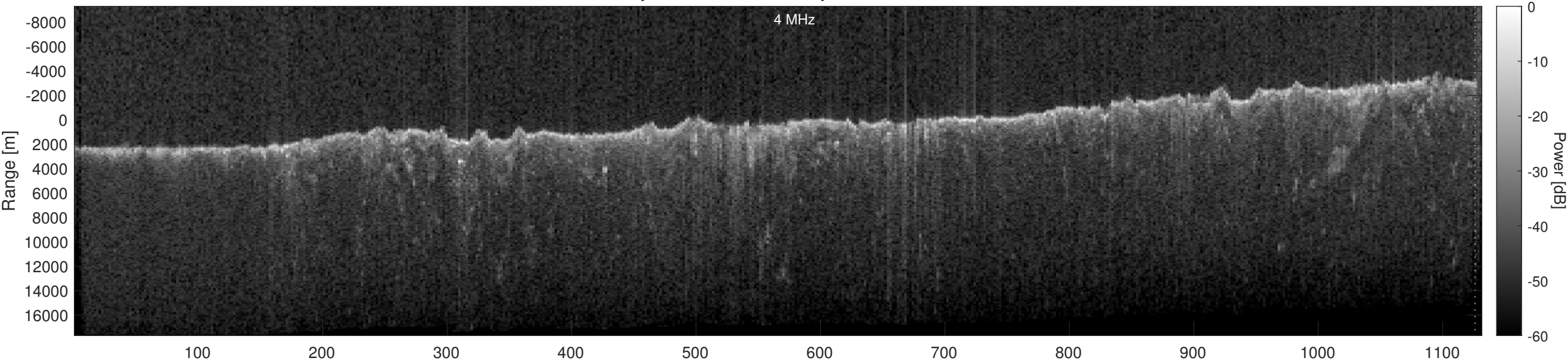
Orbit 13506, Optimized, Window, Depth-Corrected, Channel 2
