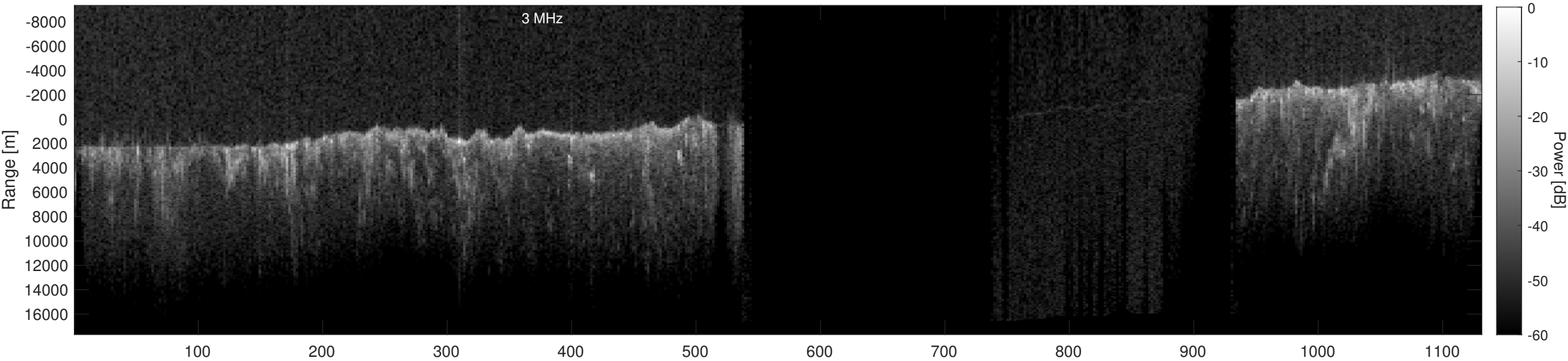
Orbit 13506, Depth-Corrected Cluttergram
