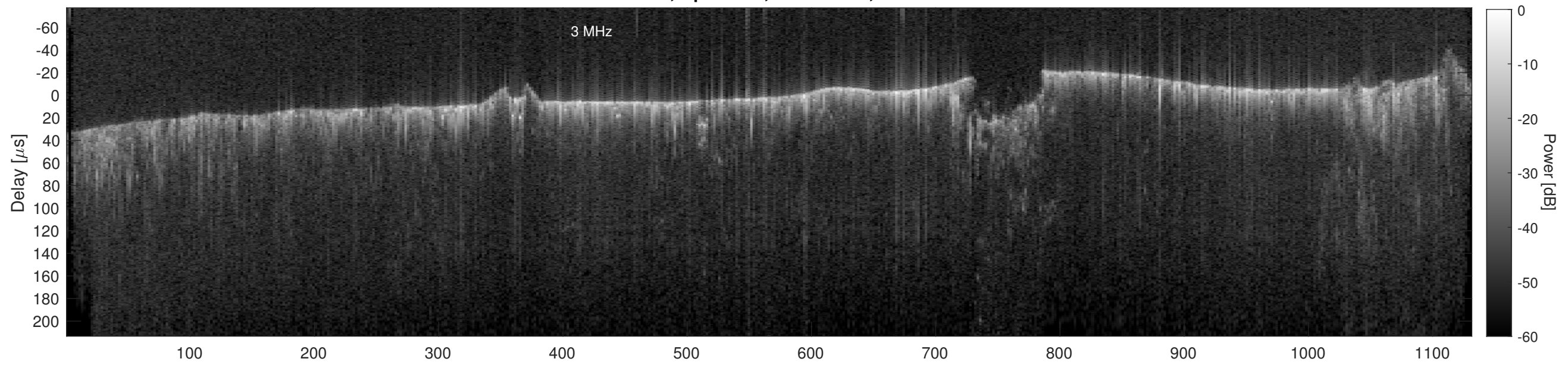
Orbit 13507, Cluttergram
