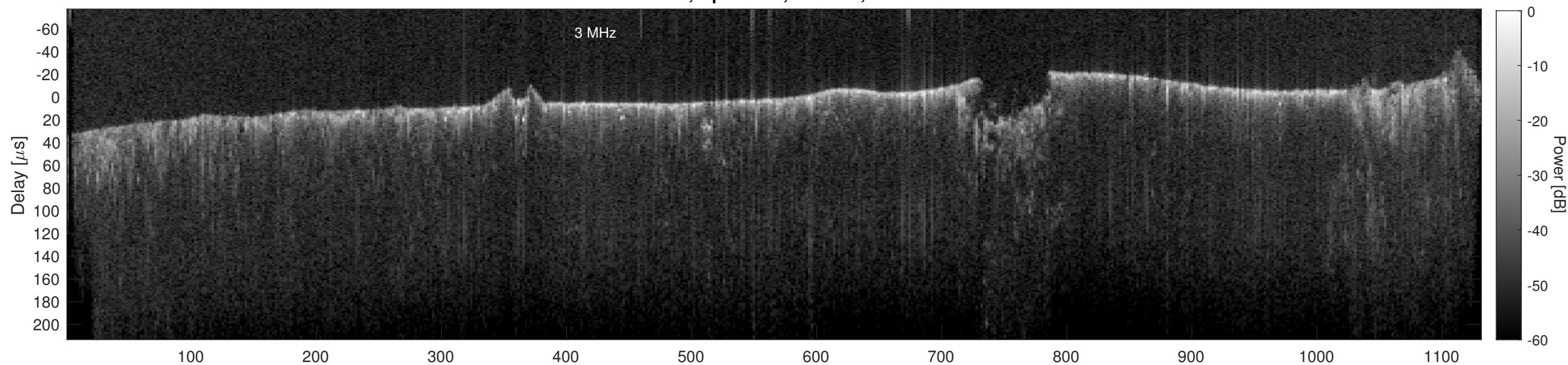
Orbit 13507, Cluttergram
