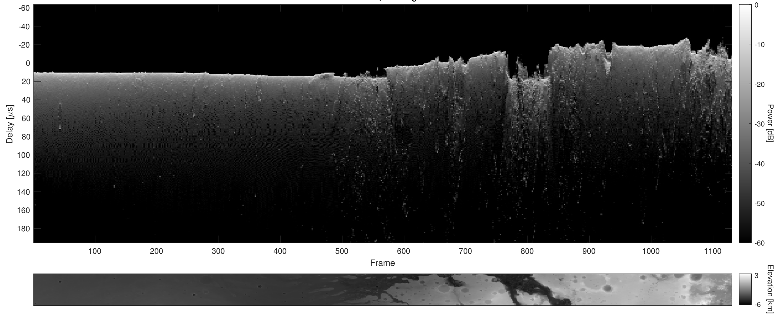
Orbit 13510, Cluttergram
