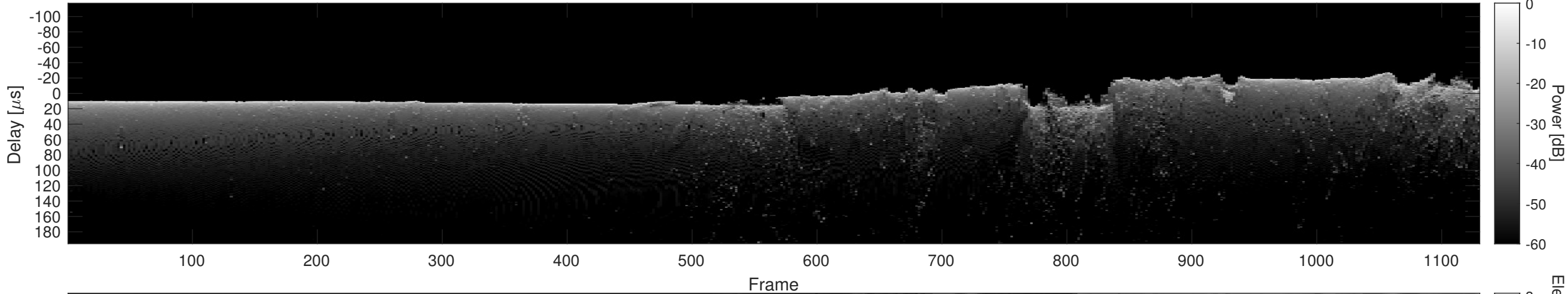
Orbit 13510, Cluttergram
