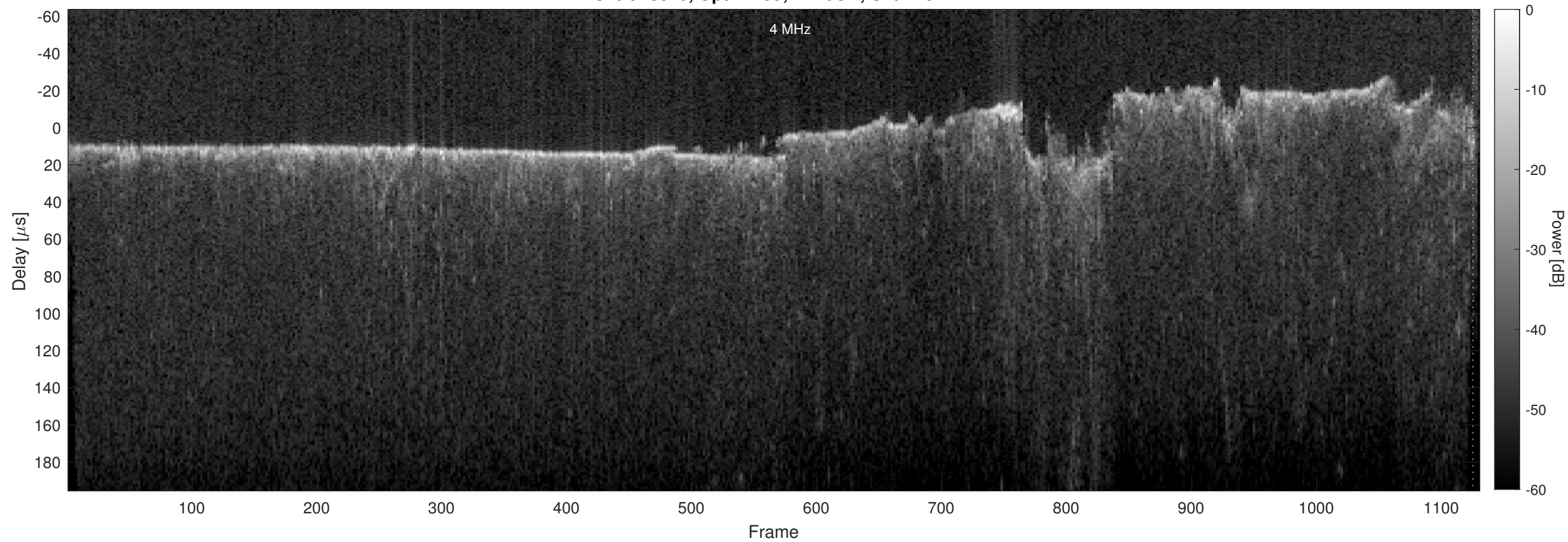
Orbit 13510, Optimized, Window, Channel 2
