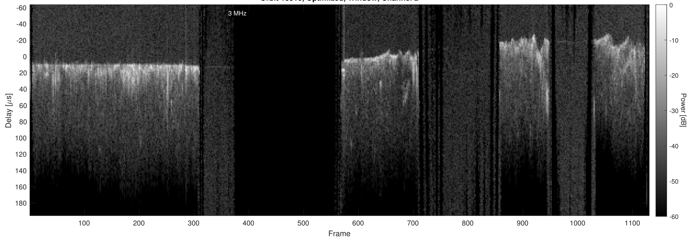
Orbit 13510, Optimized, Window, Channel 2
