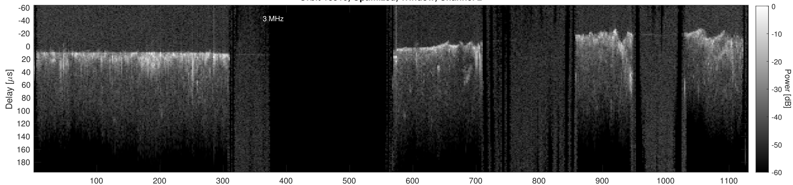
Orbit 13510, Cluttergram
