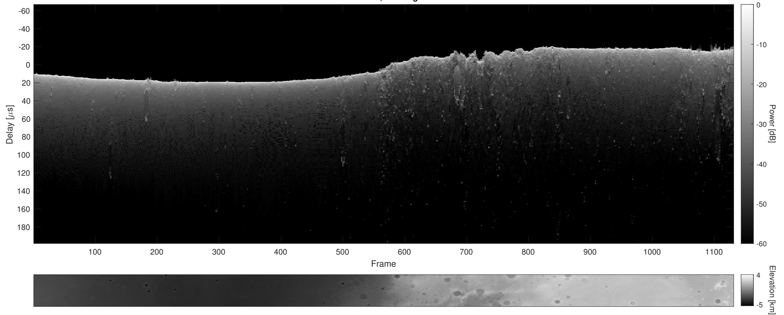
Orbit 13512, Cluttergram
