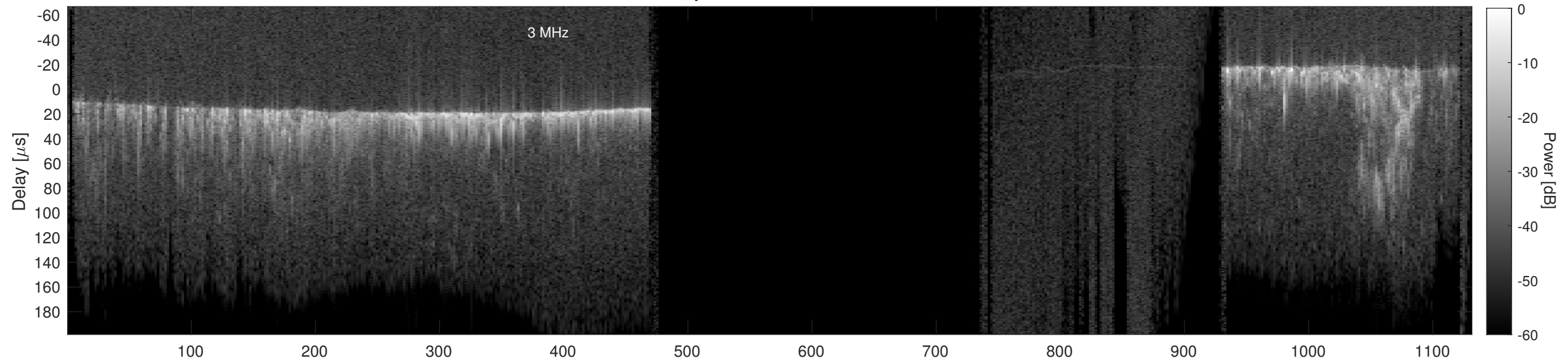
Orbit 13512, Cluttergram
