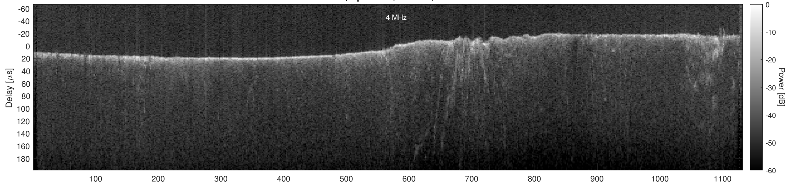
Orbit 13512, Optimized, Window, Channel 2
