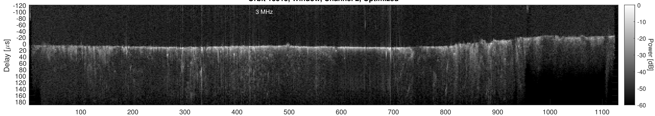
Orbit 13515, Cluttergram
