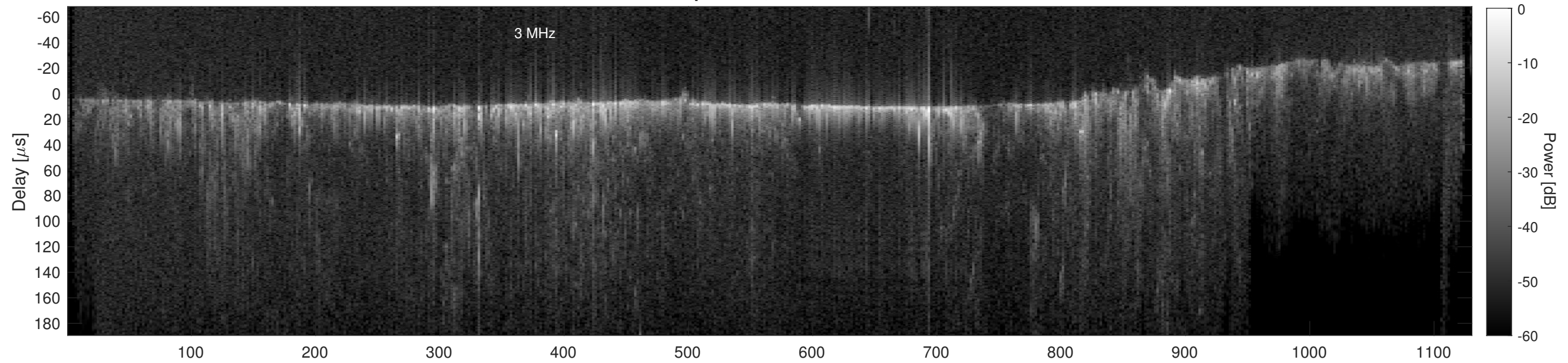
Orbit 13515, Cluttergram
