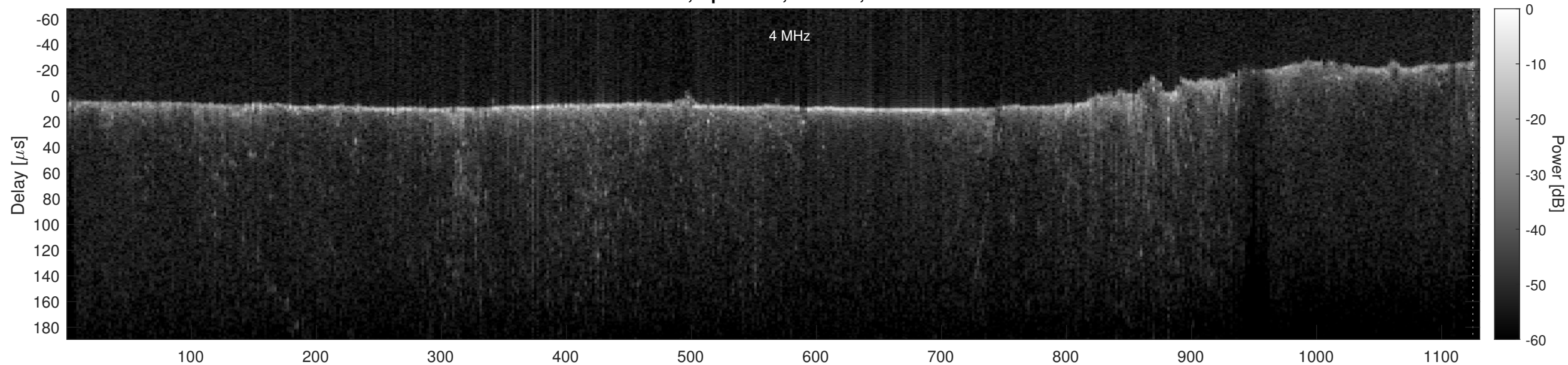
Orbit 13515, Optimized, Window, Channel 2
