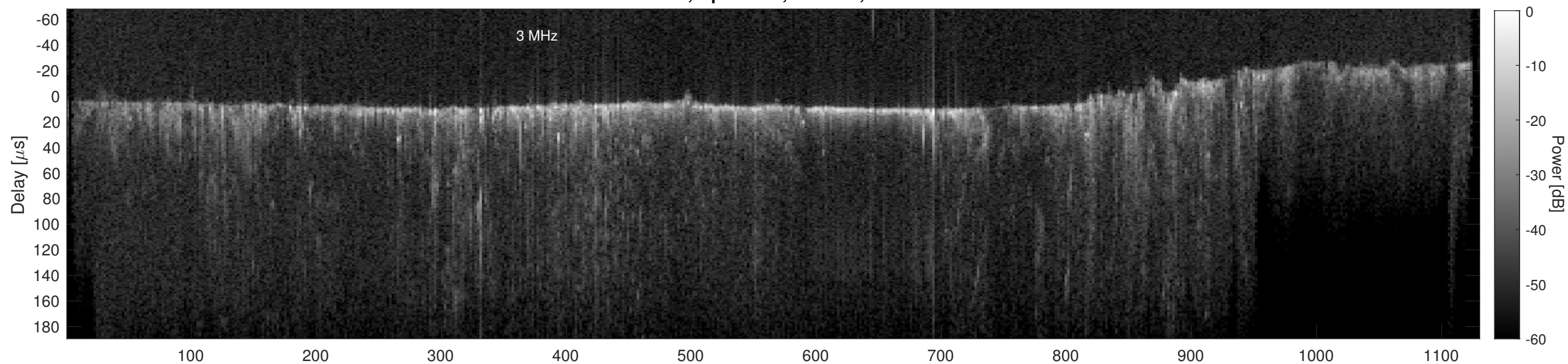
Orbit 13515, Cluttergram
