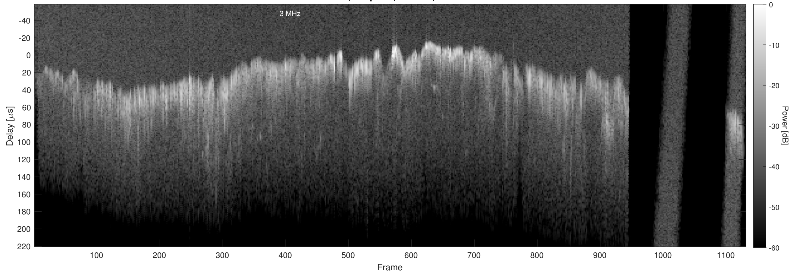
Orbit 13516, Chapman, Window, Channel 2
