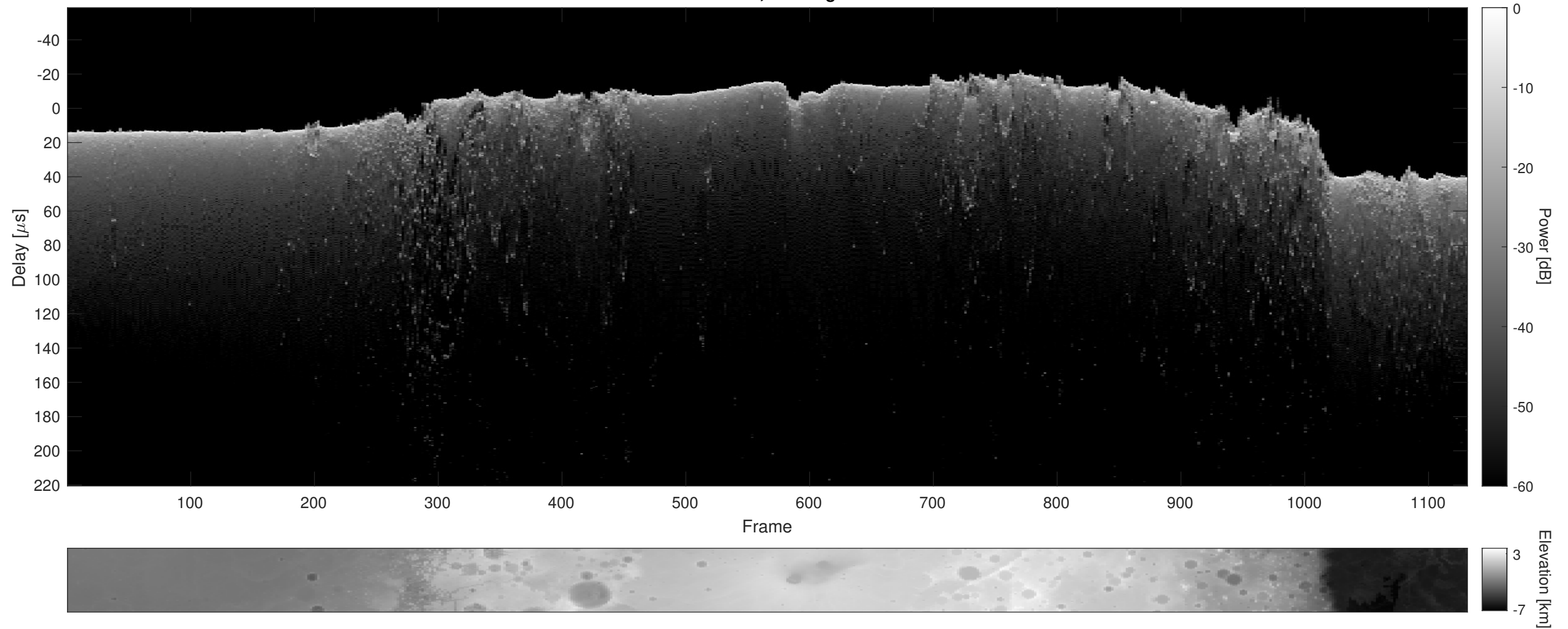
Orbit 13516, Cluttergram
