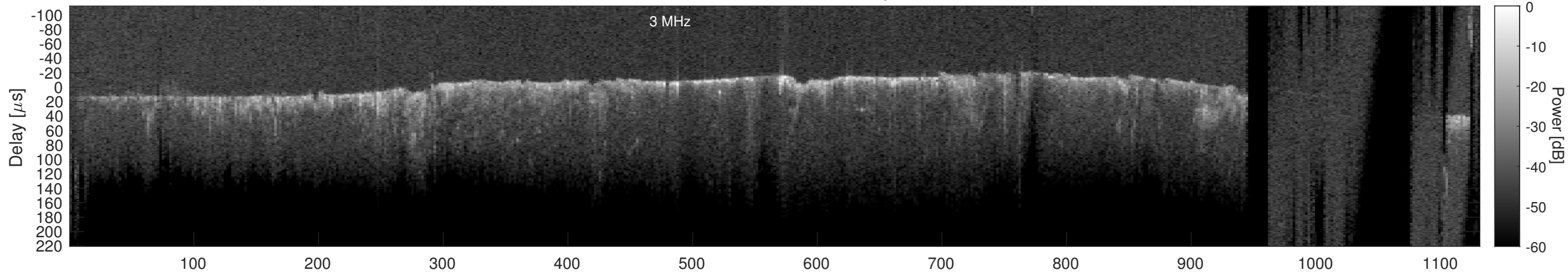
Orbit 13516, Cluttergram
