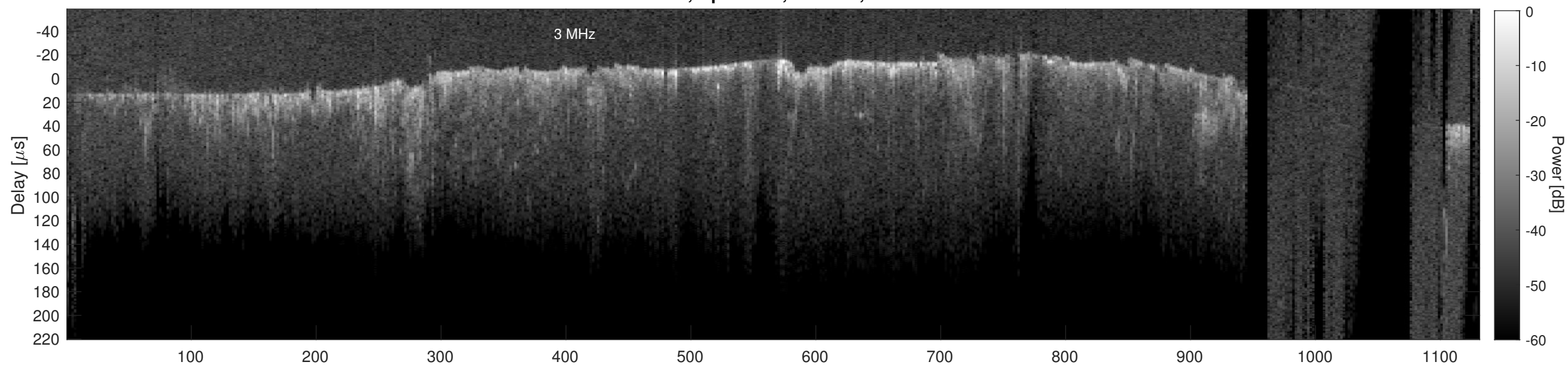
Orbit 13516, Cluttergram
