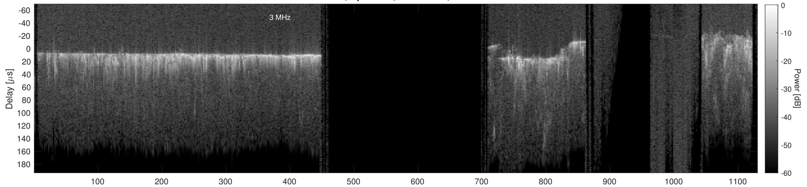
Orbit 13517, Cluttergram
