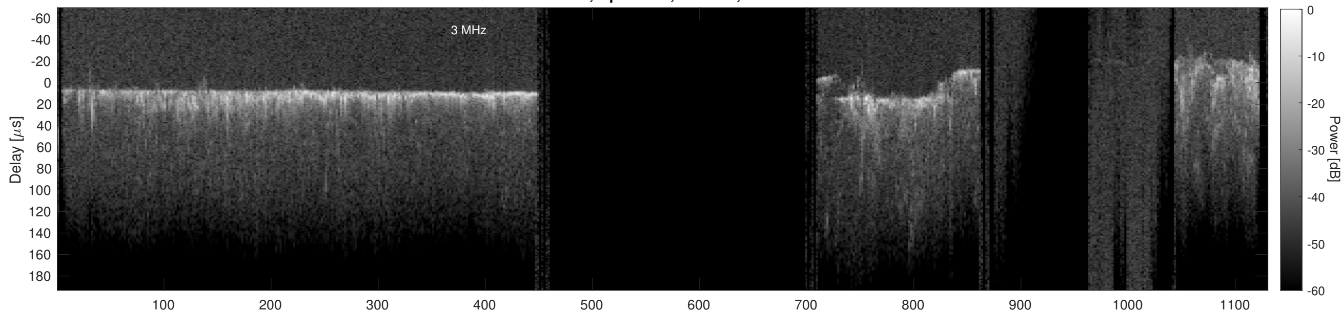
Orbit 13517, Cluttergram
